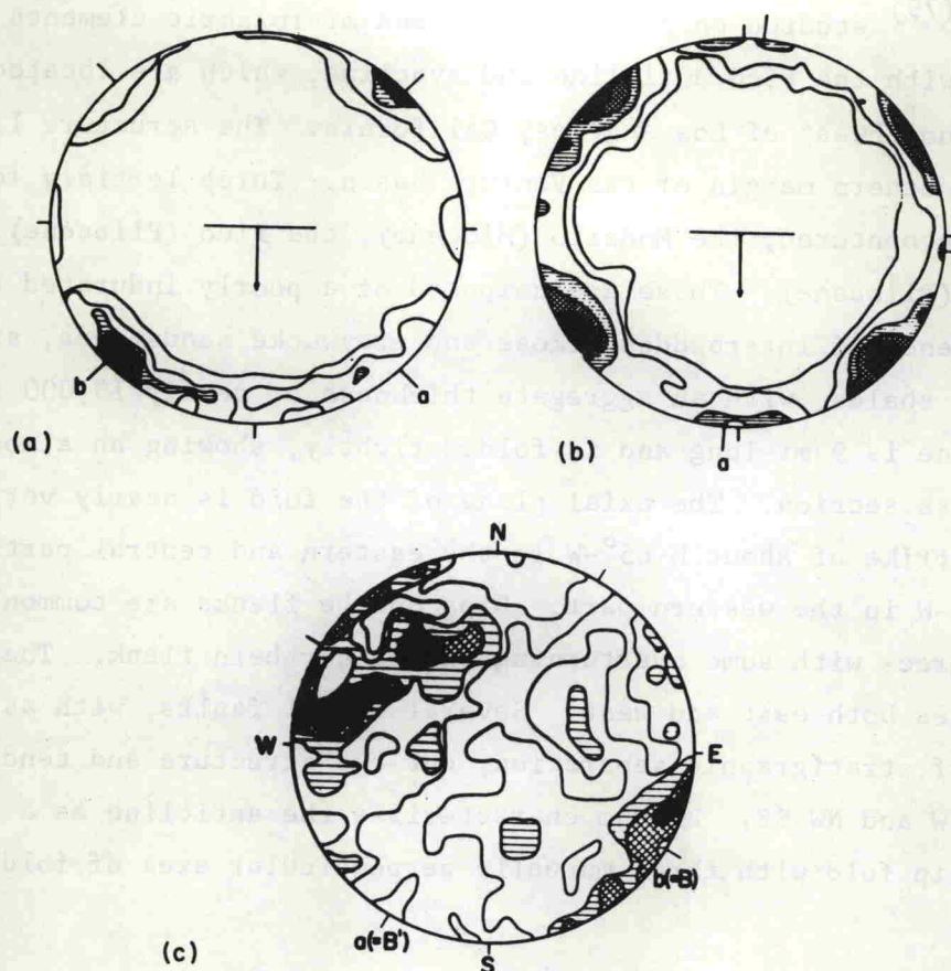
Fig. 13—Diagrams showing orientation of microfractures and macrofractures associated with the Pico structure (from Bonham, Ref. 79, Figs. 4 and 5). The plane of each diagram is parallel to bedding (ab). (a) Normals to 200 quartz microfractures. Contours are at >2, 4, 6, 8, and 10 per cent per 1 per cent area. (b) Normals to 200 quartz microfractures. Contours are at >1, 2, 4, 6, and 8 per cent per 1 per cent area. (c) Normals to 210 sets of macrofractures. Contours are at >1, 2, 3, and 4 per cent per 1 per cent area.
